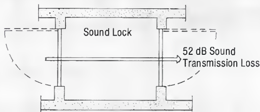
b. Sound lock doors; each door has a surface density of 10 lbs/ft²
