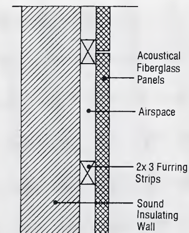
Figure 13. Furred-out surface treatment. The low frequency absorption is proportional to the airspace.
