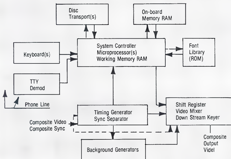
General block diagram of a practical titler for use in a broadcast situation.
