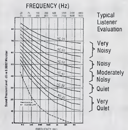
Figure 3. Noise criterion (NC) curves
