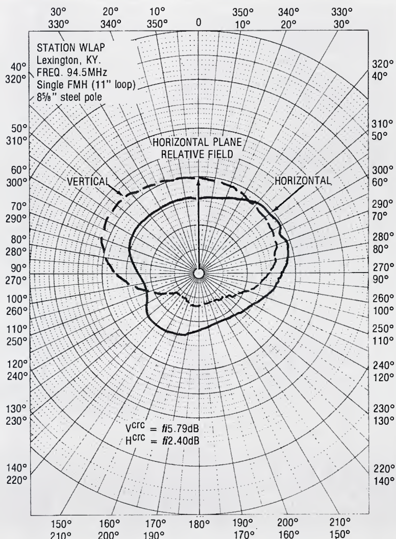
Antenna pattern without optimization
