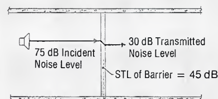
Figure 4. Sound Transmission Loss (STL) is the measure of reduction of airborne sound through a barrier.
