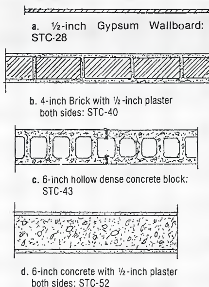
Figure 6. STC ratings of typical homogeneous walls
