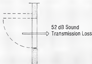
a. Single door; door has a surface density of 100lbs/ft²
